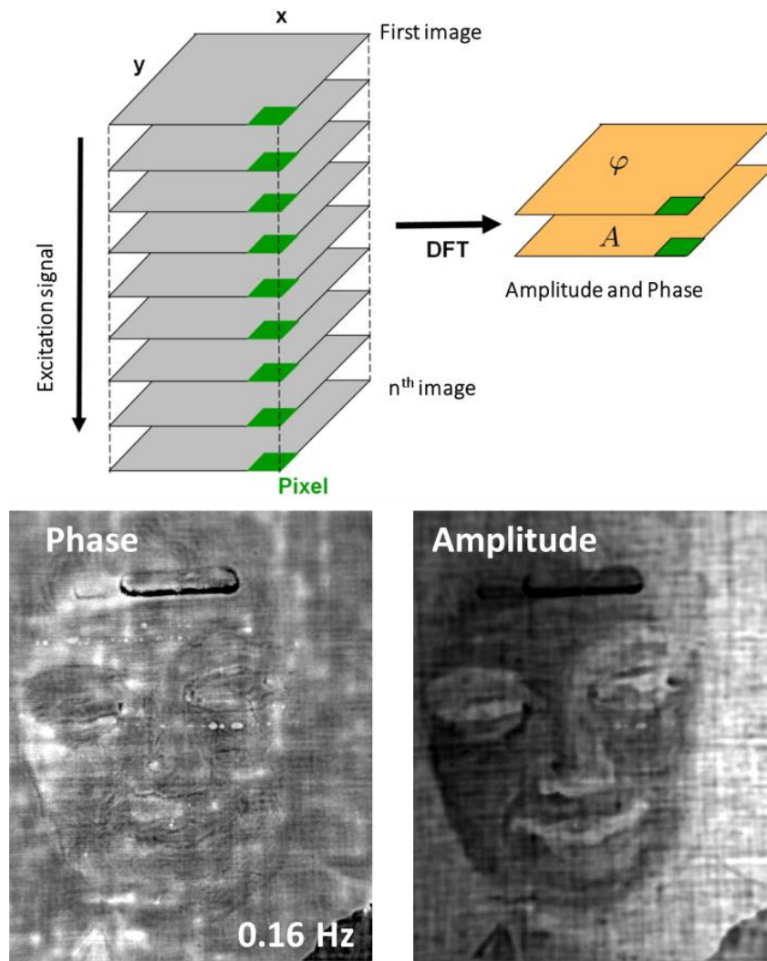
Figure 4. Workflow of the Pulse-phase-thermography used by DisplayImg Professional software. The example of phase and amplitude images computed by the software for \nu = 0.16 Hz for a distance between the painting and the camera of one meter.
